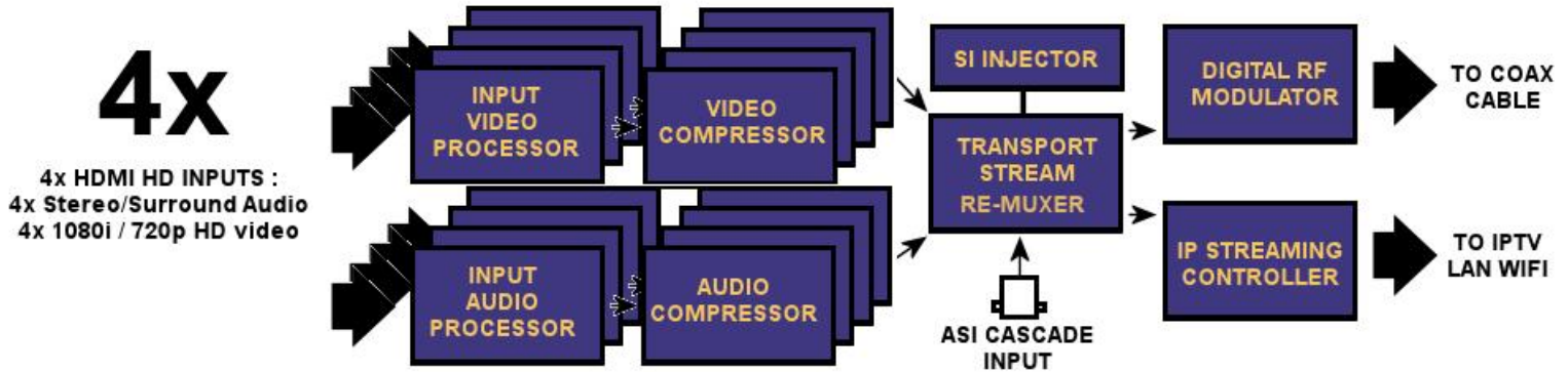
BLOCK DIAGRAM
